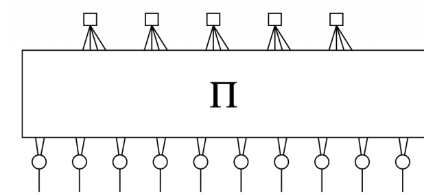
Figure 4: Graphical representation of an LDPC code as a concatenation of SPC and REP codes. \pi represents an interleaver.
